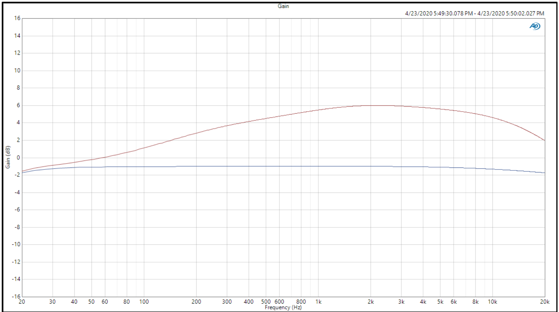
Fretless Contour – trim pots centered
